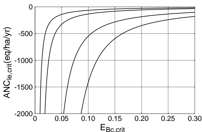
Figure 2-2: Critical ANC leaching (as defined by eq.2.27, for Q=1 m/a) as a function of the critical base saturation, E_{Bc,crit} for [Bc]=0.02 eq/m 3 , K_{gibb}=10^8 and K_{Gap}=0.005 (leftmost curve), 0.01, 0.03 and 0.05 (rightmost curve). (To obtain ANC_{Le,crit} for arbitrary Q , multiply the values on the vertical axis by Q in m/a; see also Figure 2-4 below.)
