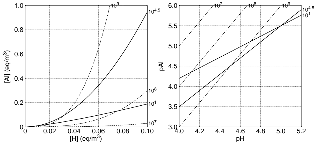
Figure 2-3: Relationships between proton and Al concentration in \text{eq/m}^3 (left) and in their logarithmic forms (right) for K_{Al_{ox}} = 10^1 , a=2 and K_{Al_{ox}} = 10^{4.5} , a=1.3 (solid lines) as well as three gibbsite equilibria ( a=3 ) with K_{gibb} = 10^7 , 10^8 and 10^9 (dashed lines). Note: [H] = 0.1 \text{ eq/m}^3 corresponds to pH = 4 .
