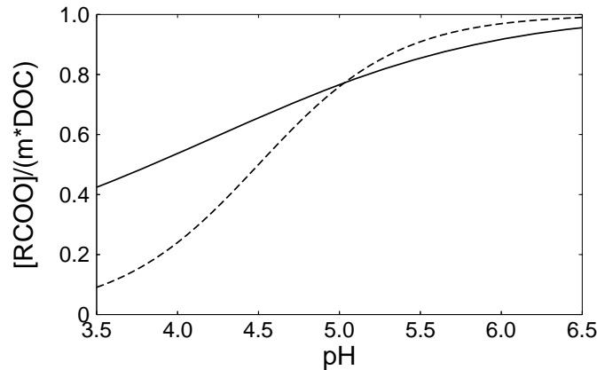
Figure 2-5: Fraction of organic acids ( m\text{-DOC} ) dissociated as a function of pH for the Oliver model (solid line) and the mono-protic model (eq.2.45) with pK_1=4.5 (dashed line).
