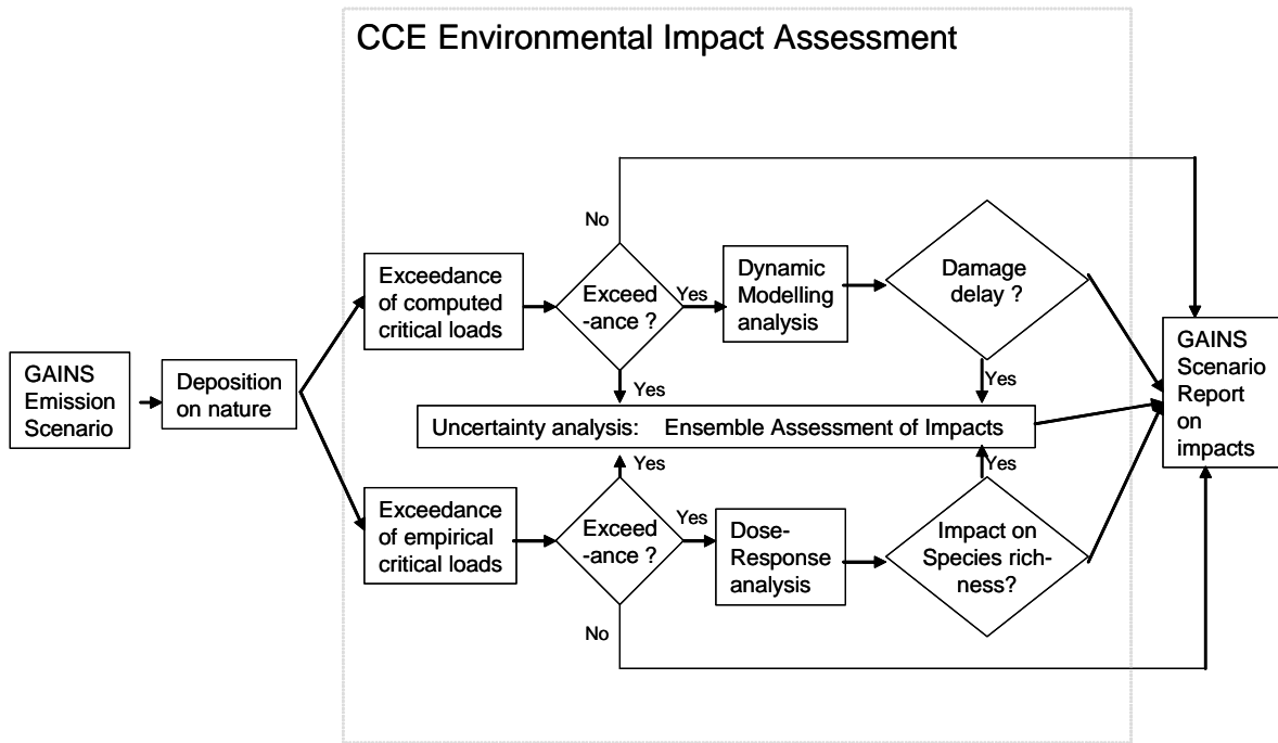
Figure 1-1 Schematic overview of the CCE Environmental Impact Assessment (CCE-EIA) methodology in the context of EC4MACS for the analysis and comparison of impacts relative to GAINS scenarios.
